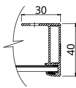
Frame Cross Section A-A
